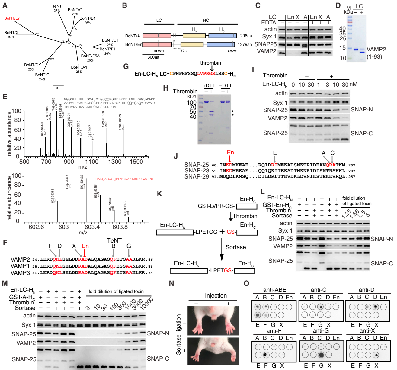
Figure 1. BoNT/En Is a Unique BoNT Serotype and Cleaves VAMP2 and SNAP-25 in Neurons
