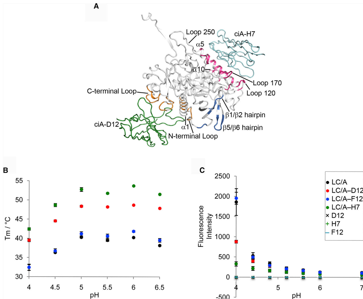
Figure 4. VHH ciA-H7 Interferes with Low-pH-Triggered LC/A Unfolding
