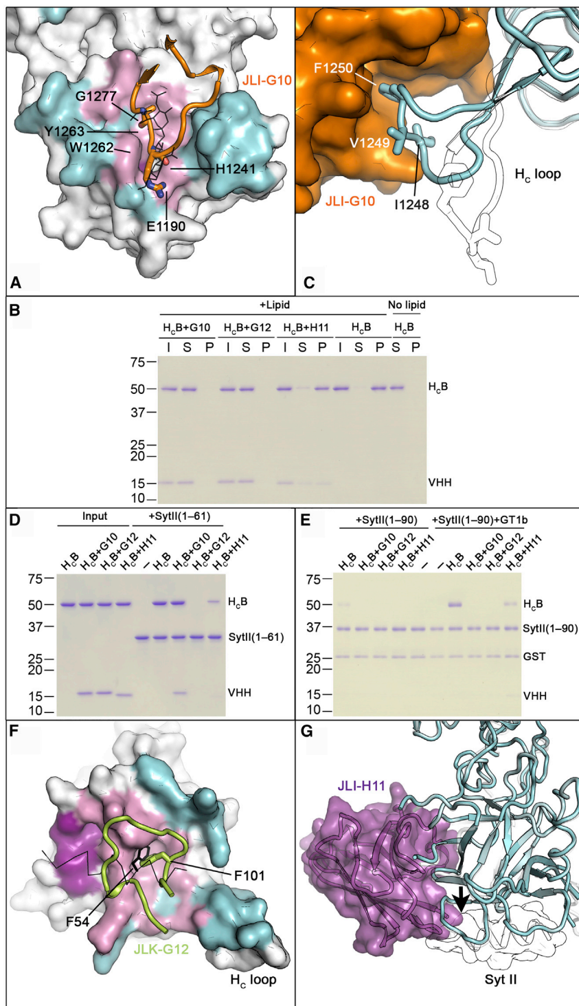
Figure 2. VHHs JLI-G10, JLK-G12, and JLI-H11 Inhibit H c B Binding to Host Receptors
