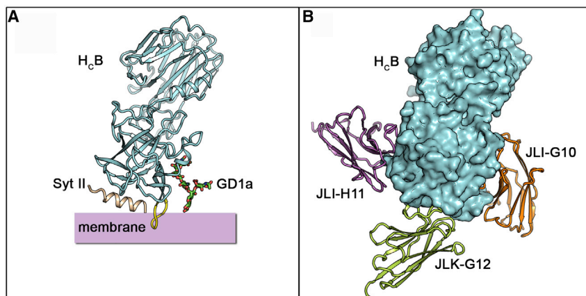
Figure 1. Structures of H C B in Complex with JLI-G10, JLK-G12, or JLI-H11
